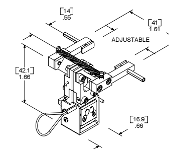
MODEL 3475 WITH ±1 MM MEASURING RANGE
