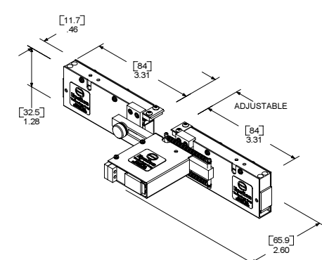
MODEL 3560 DIMENSIONS: [mm] inches
