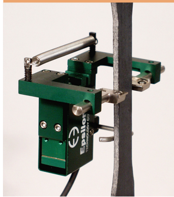
Model 3575 extensometer
